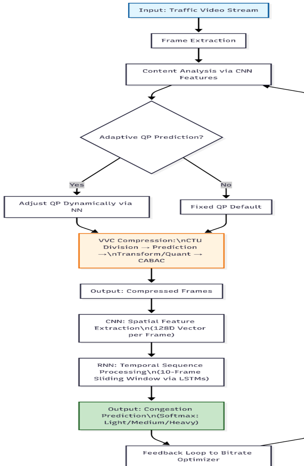
Figure 1. Flowchart of the Proposed VCM Algorithm
