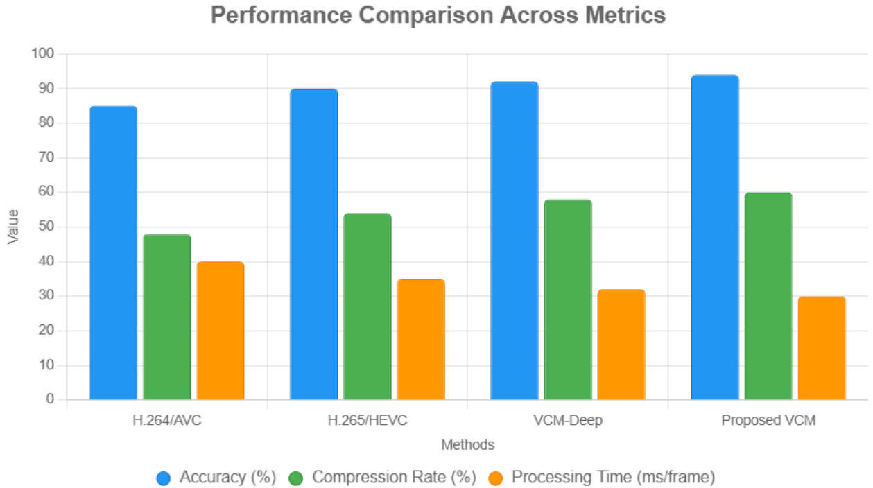
Figure 2. The Bar Chart of Performance Metrics with Error Bars (SD)
