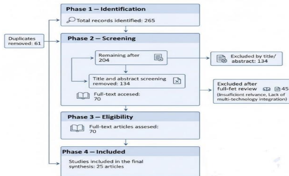
Figure 1. PRISMA Flow Diagram of the Methodology
