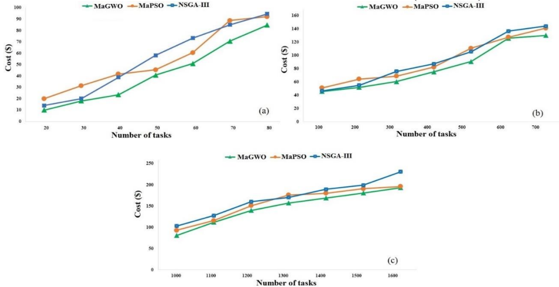
Figure 7. Task Execution Costs Based on Task Types: a- Number of Small-Sized Tasks; b- Number of Medium-Sized Tasks; c- Number of Large-Sized Tasks
