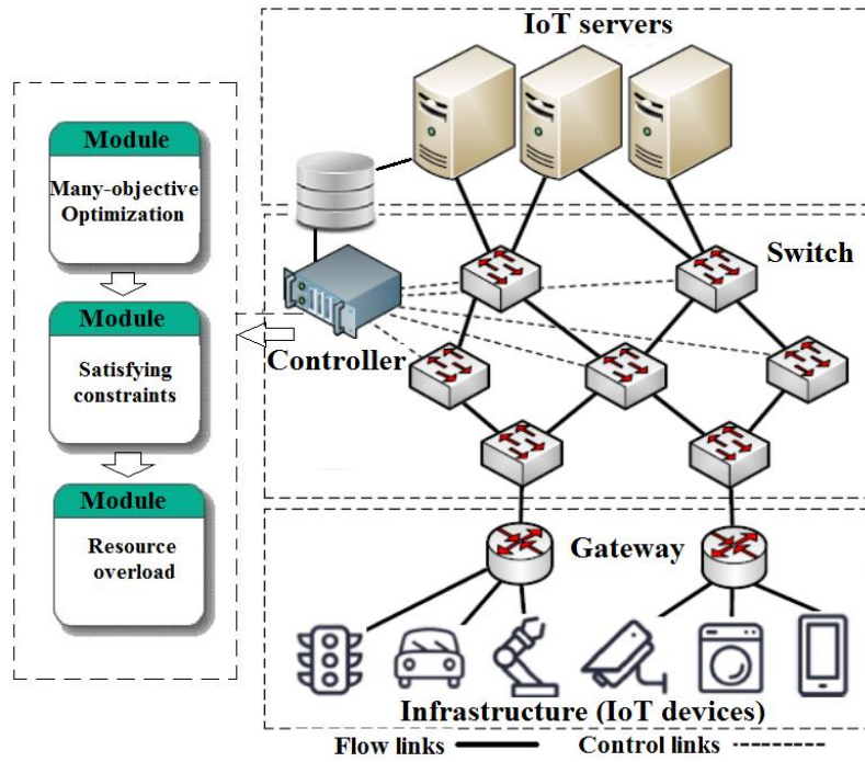
Figure 1. The Proposed Framework Considering QoS Improvement and Load Balancing
