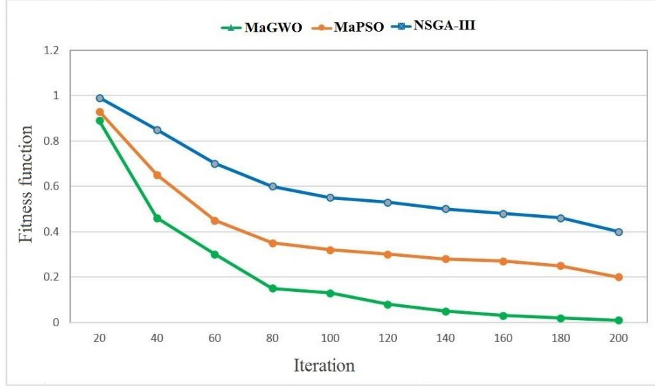
Figure 7. Convergence Chart Over 200 Iterations
