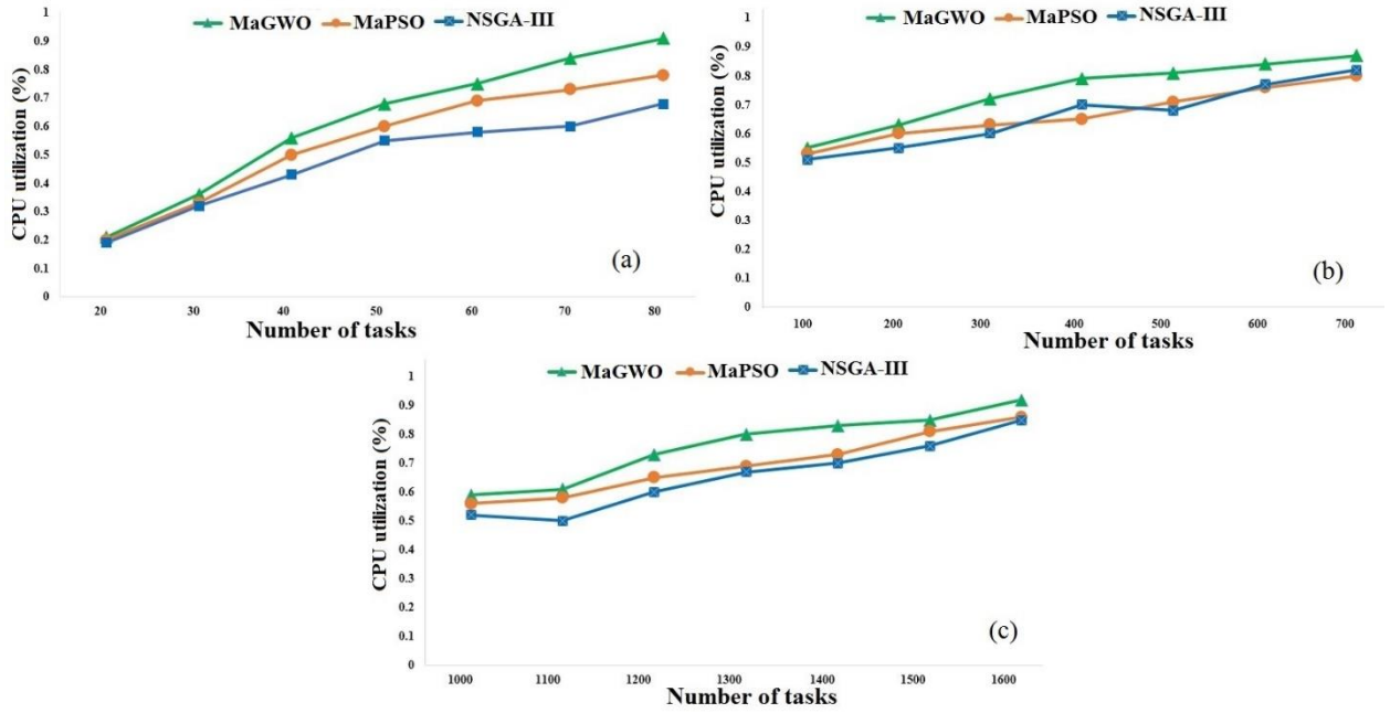
Figure 6. Comparative Results Based on Resource Utilization for Different Task Types: a- Number of Small-Sized Tasks; b- Number of Medium-Sized Tasks; c- Number of Large-Sized Tasks
