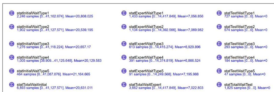
Figure 10. Simulation Results for Scenario 1 – Statistics Elements Output
